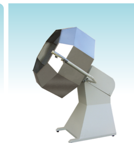
TW-II八角调味机 Eight Square Flavoring Machine
