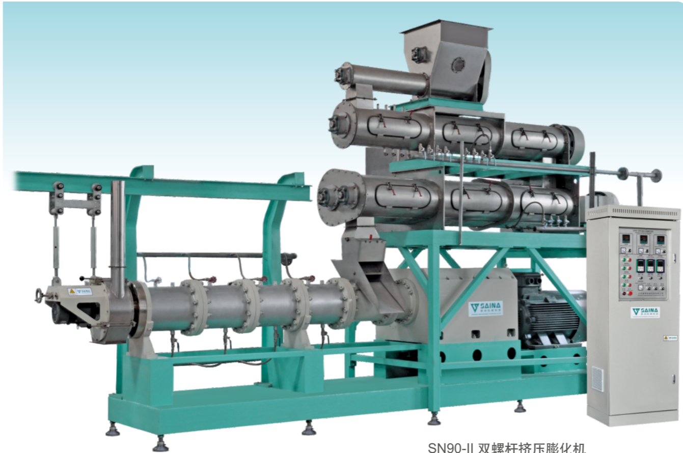
SN90-II 双螺杆挤压膨化机 SN90-II Double-screw Extruder
